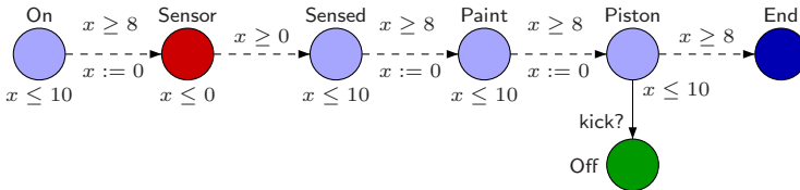
Fig. 1. Timed Game with Imperfect Information
