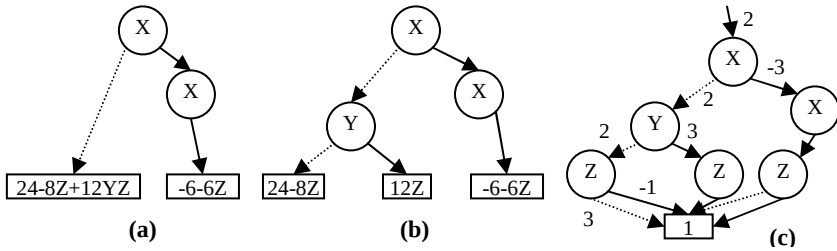
Fig. 2. LTED representation of 24 \cdot 8 \cdot Z + 12 \cdot Y \cdot Z - 6 \cdot X^2 - 6 \cdot X^2 \cdot Z (a) decomposition with respect to variable X (b) decomposition with respect to variables X and Y (c) decomposition with respect to variables X , Y and Z
