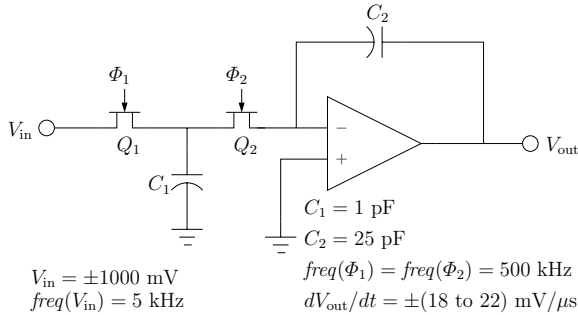
Fig. 1. Circuit diagram of a switched capacitor integrator
