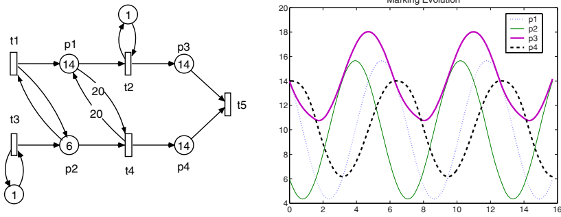
Fig. 5. A TCPN and its marking evolution with \lambda = [1, 10, 10, 20, 1] . The system switches indefinitely, and does not approach a limit marking.
