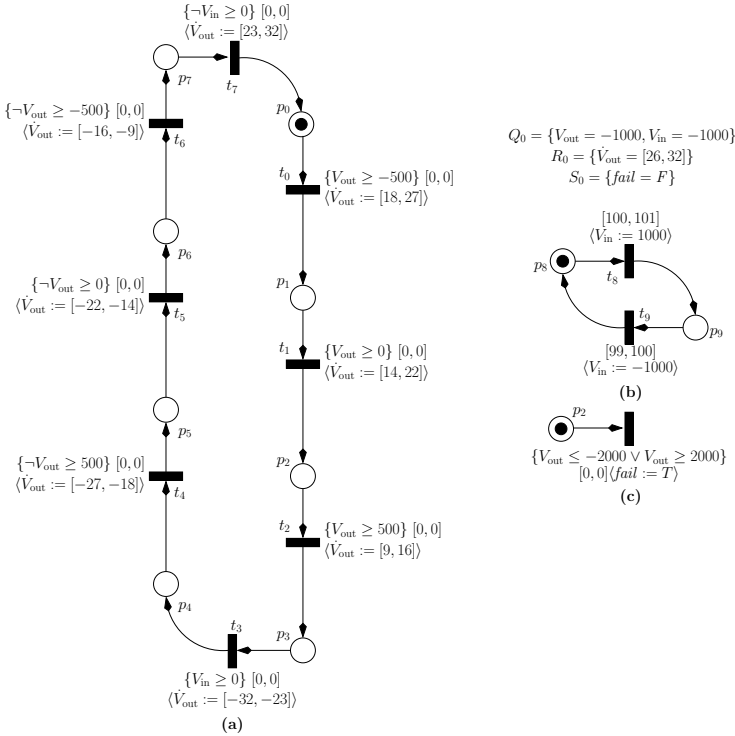
Fig. 6. LHPN for the corrected switched Integrator Example
