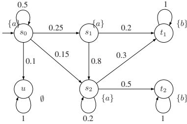
Fig. 2. \text{unif}(\mathcal{C}) = \mathcal{U}
